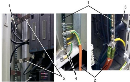
Fig. 11. Design of communication system cabinet grounding 1 – potential equalizer bar; 2 – external grounding system cable; 3 – insulator insulating the potential equalizer bar from the cabinet body; 4 – elements connecting the potential equalizer bar with the cabinet body; 5 – flexible links connecting the electronic devices enclosures with the potential equalizer bar.
