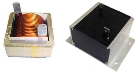
Fig. 9. Chokes manufactured by CWS with a helical coil and a core made of the special alloy attenuating the electromagnetic pulse in the power supply cable. Left – open, right – encapsulated in epoxide compound
