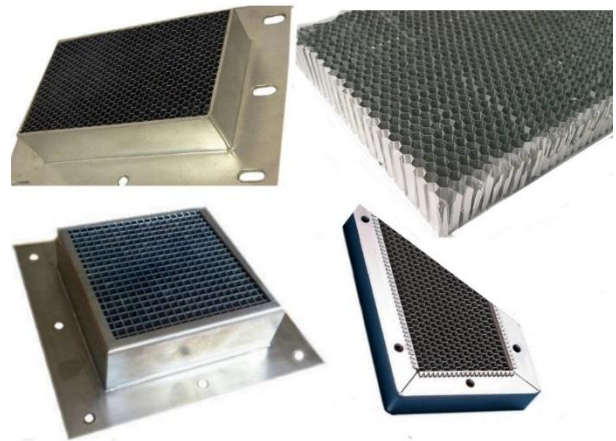
Fig. 5. Ventilating honeycomb panels
