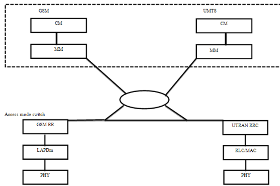
Figure 3: Access Mode Switching of MHNb (protocols adapted from [11] and [12])
