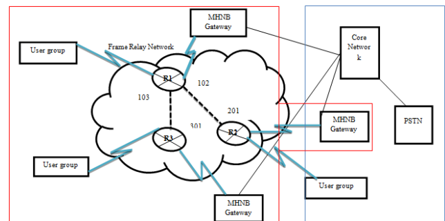
Figure 6: Interconnection between MHNb Network, Core Network and other Public Switch Telephone Network (PSTN).
